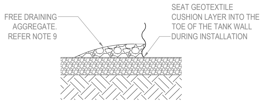
TANK WALL DETAIL
